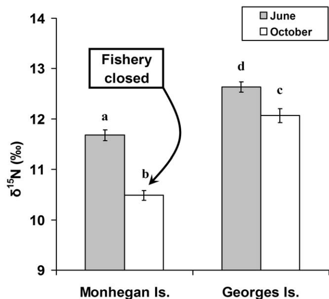
Figure 1. The effects of herring bait on the diet of lobsters in coastal Maine. Nitrogen stable isotope ratios [SIR's] for sublegal (66–83 CL) lobsters in the summer and fall from closed and open sites in mid-coast Maine ( n = 10 ; error bars = \pm 1 SE). ANOVA revealed a significant interaction between site and season. Nitrogen SIR's of Monhegan lobsters were significantly lower in October than in June, but did not differ at the baited (GI) site. Higher \delta^{15}\text{N} values for lobsters indicate greater proportions of higher trophic levels such as herring in their diet. doi:10.1371/journal.pone.0010188.g001
