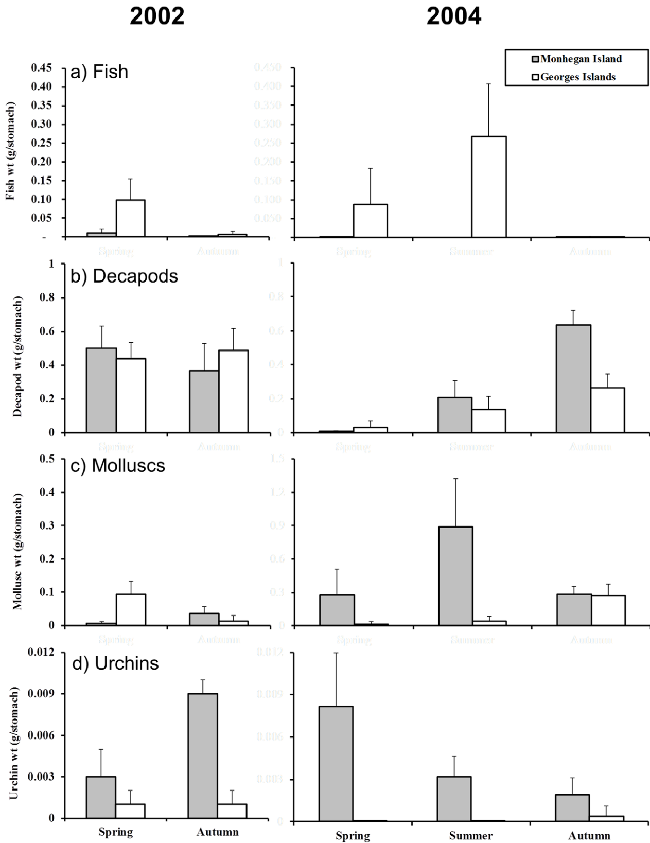
Figure 3. The diet composition of lobsters from Monhegan and Georges Islands. The effects of season (spring and autumn in 2002; spring, summer and autumn in 2004) and site (Monhegan Island vs. the Georges Islands) on a) fish, b) decapod, c) mollusc, and d) urchin biomass found in stomach contents of lobsters (n=20 in 2002; n=8–10 in 2004; error bars =+1 SE). doi:10.1371/journal.pone.0010188.g003
