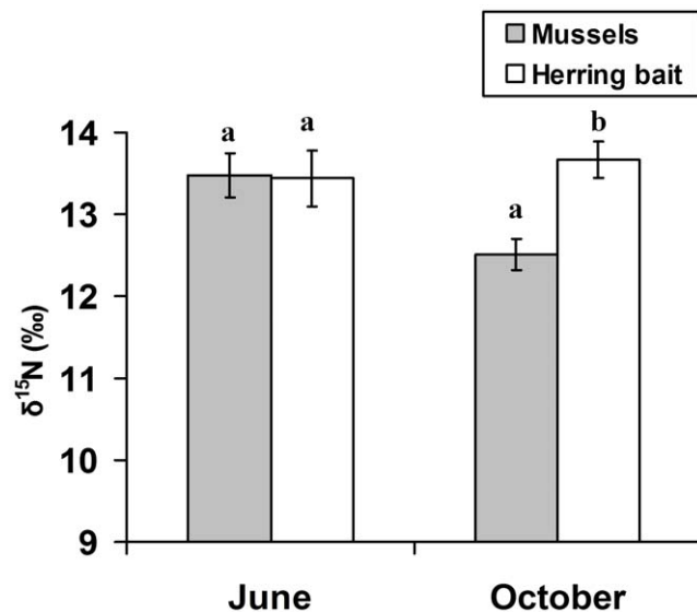
Figure 2. The effects of herring bait on lobster N SIR values. N SIR values of lobsters reared on herring bait ( n = 5 ) vs. mussels ( n = 6 ) in the laboratory at the Darling Marine Center (error bars = +1 SE). N SIR values were similar at the start (June) of the experiment, but lobsters that consumed mussels were significantly lower at the end (October) of the experiment. Letters denote the results of Ryan's Q post hoc tests—bars with different letters were significantly different at p < 0.05 . doi:10.1371/journal.pone.0010188.g002
